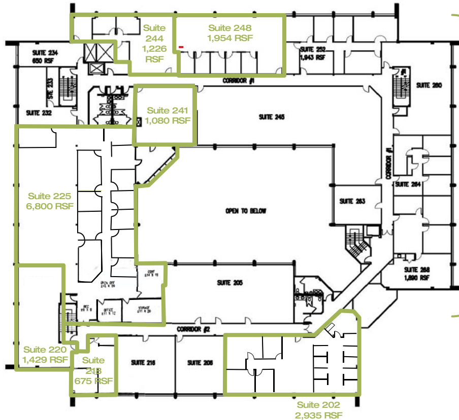
Second Floor
